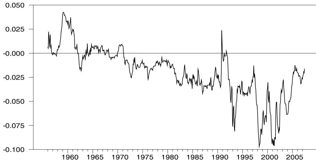
Figure 3. The risk premium is estimated for the entire 1946-2007 sample using 10 years of data for each estimate. Thus, the first period starts in 1956. We update the estimates each month by dropping the earliest observation and adding the latest observation.
