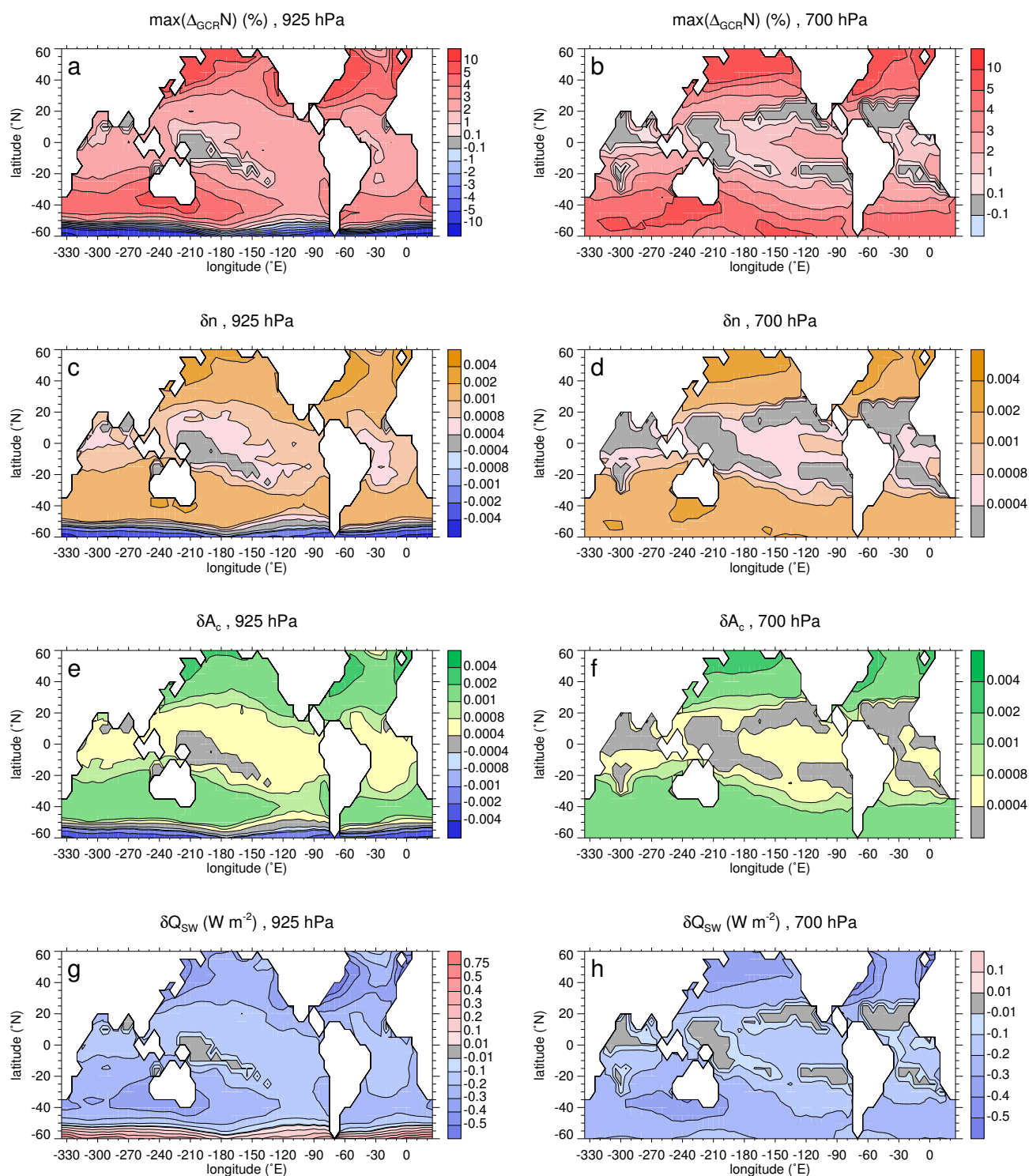
Fig. 12. Spatial distributions of \max(\Delta_{\text{GCR}} N) ( a , b ), and of the resulting change in cloud fraction \delta n ( c , d ), cloud albedo \delta A ( e , f ), and in the daily mean shortwave radiative forcing \delta Q_{\text{SW}} ( g , h ) for aerosol that nucleated at the 925 hPa (left) and 700 hPa (right) levels, on 21 March.
