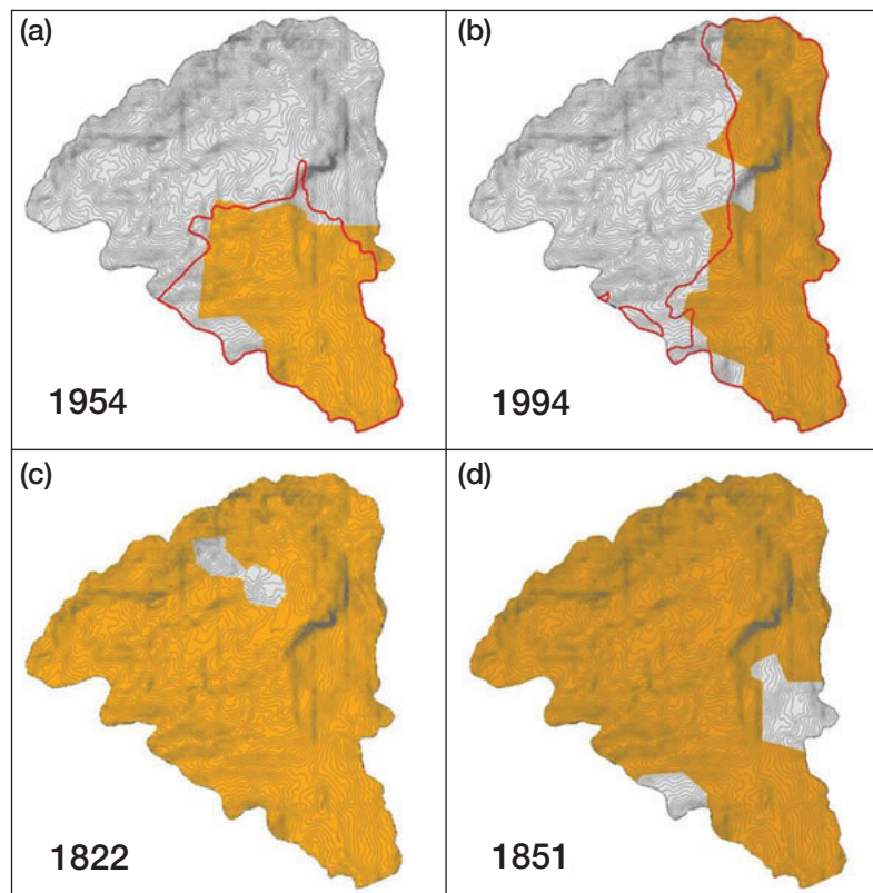
Figure 4. Fire perimeters in the Rincon Mountains, Arizona, reconstructed from a 2780-ha fire-scar network. (a and b): Shaded polygons represent fire areas in 1954 and 1994 reconstructed from fire scars; red outline indicates National Park Service-mapped fire perimeters. (c and d): Shaded polygons represent fire areas for 1822 and 1851, reconstructed from fire scars based on the same interpolation algorithm. Derived from Farris et al. (2010).
