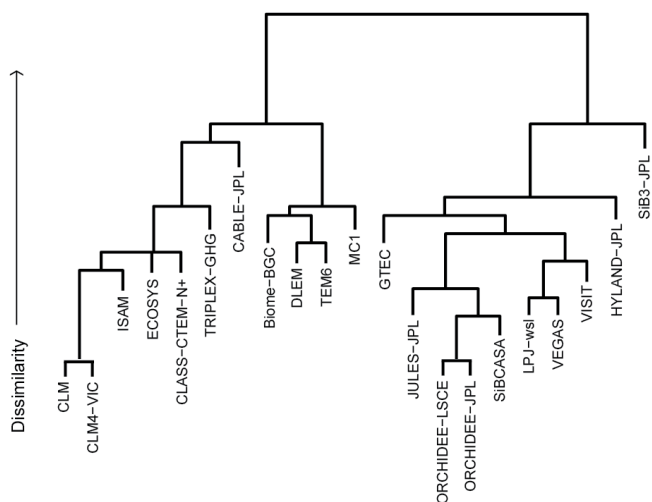
Fig. 2. Dendrogram showing overall model structural differences determined by Hamming distance for the models participating in MstMIP. Models in the same “tree” share similar structural model characteristics. For example, models in the “tree” to the left include an explicit nitrogen cycle, while models in the “tree” to the right do not. Models are further separated or clustered by their treatment of soil carbon pools (e.g., SiB3-JPL does not include live, soil, or litter carbon pools) and their treatment of radiation and canopy heat storage (e.g., Biome-BGC, DLEM, TEM6, and MC1 do not account for canopy heat storage, nor partition radiation into latent and sensible heat). Refer to the Supplement for the binary data used to create this diagram.
