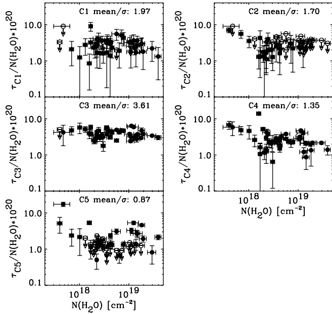
FIG. 16.—Peak optical depths of the 5–8 μm components (Fig. 8), normalized to N(\text{H}_2\text{O}) , plotted as a function of N(\text{H}_2\text{O}) . Error bars are 1 \sigma , but open symbols with arrows attached refer to 3 \sigma upper limits. At the top right of each panel the ratio of the mean over the standard deviation of the sample (excluding upper limits) is indicated. Component C3, i.e., the short-wavelength component of the 6.85 μm feature, correlates significantly better with N(\text{H}_2\text{O}) than the other components do. Of the components that produce the 6.0 μm excess, C1 correlates better with \text{H}_2\text{O} than does C5. Note the increased strengths of C2 and C4 at low N(\text{H}_2\text{O}) .
