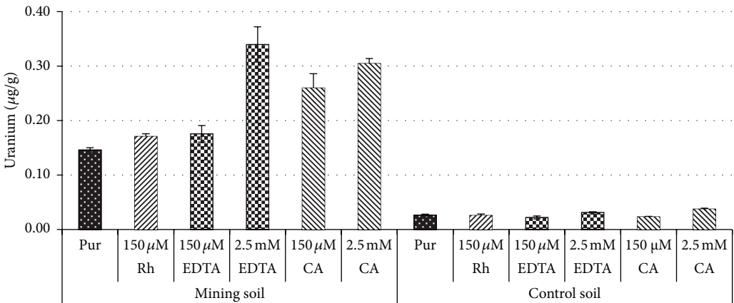
FIGURE 2: Removal of uranium from the mining and control soils utilizing rhamnolipid ( 150\ \mu\text{M} ), EDTA ( 150\ \mu\text{M} and 2.5\ \text{mM} ), and citric acid ( 150\ \mu\text{M} and 2.5\ \text{mM} ). Pur: purified water ( 18\ \text{M}\Omega\cdot\text{cm} ), Rh: rhamnolipid, and CA: citric acid.
