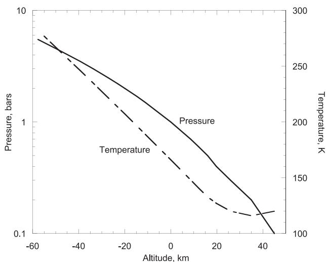
Figure 1. Atmospheric pressure and temperature as functions of altitude from Seiff et al. [1998].
